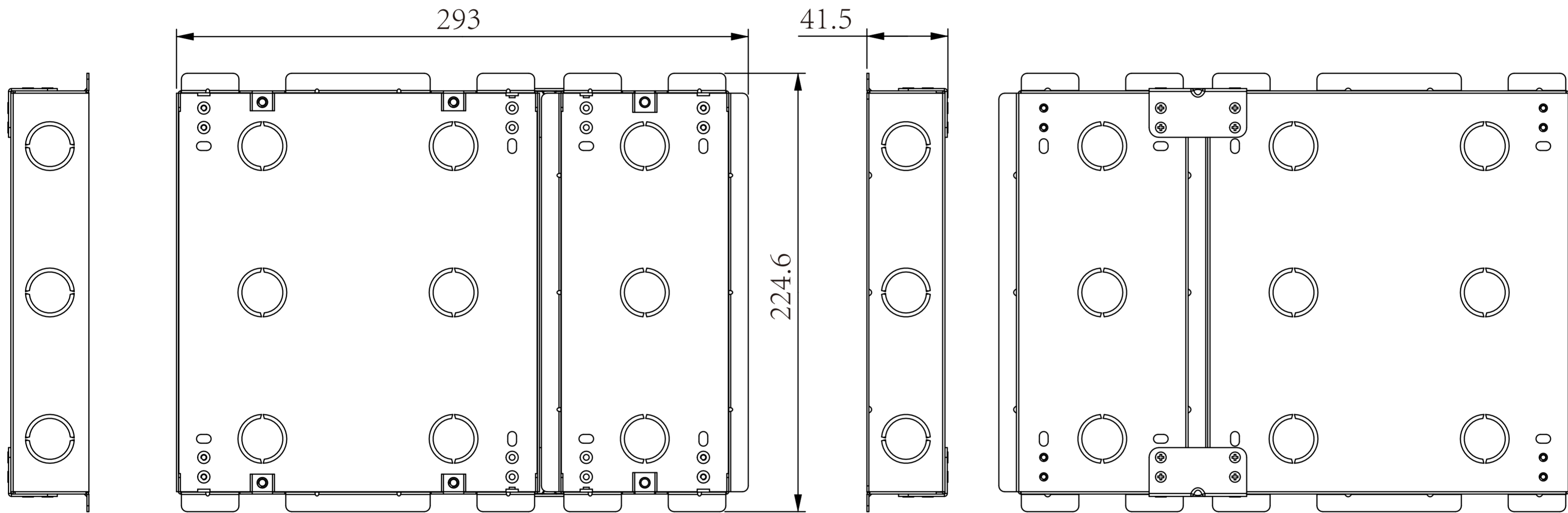
② RIGHT VIEW
