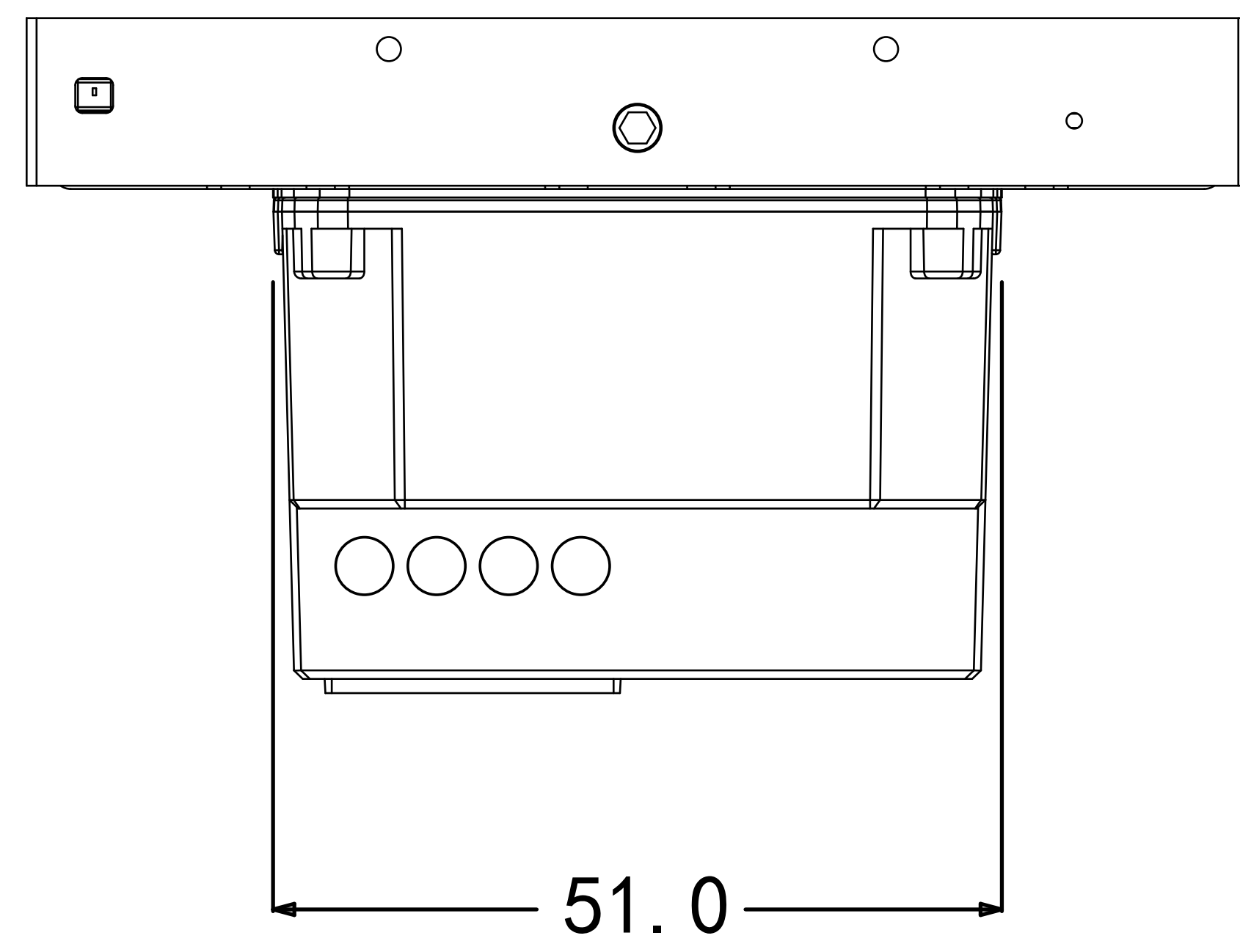
5 BOTTOM VIEW
