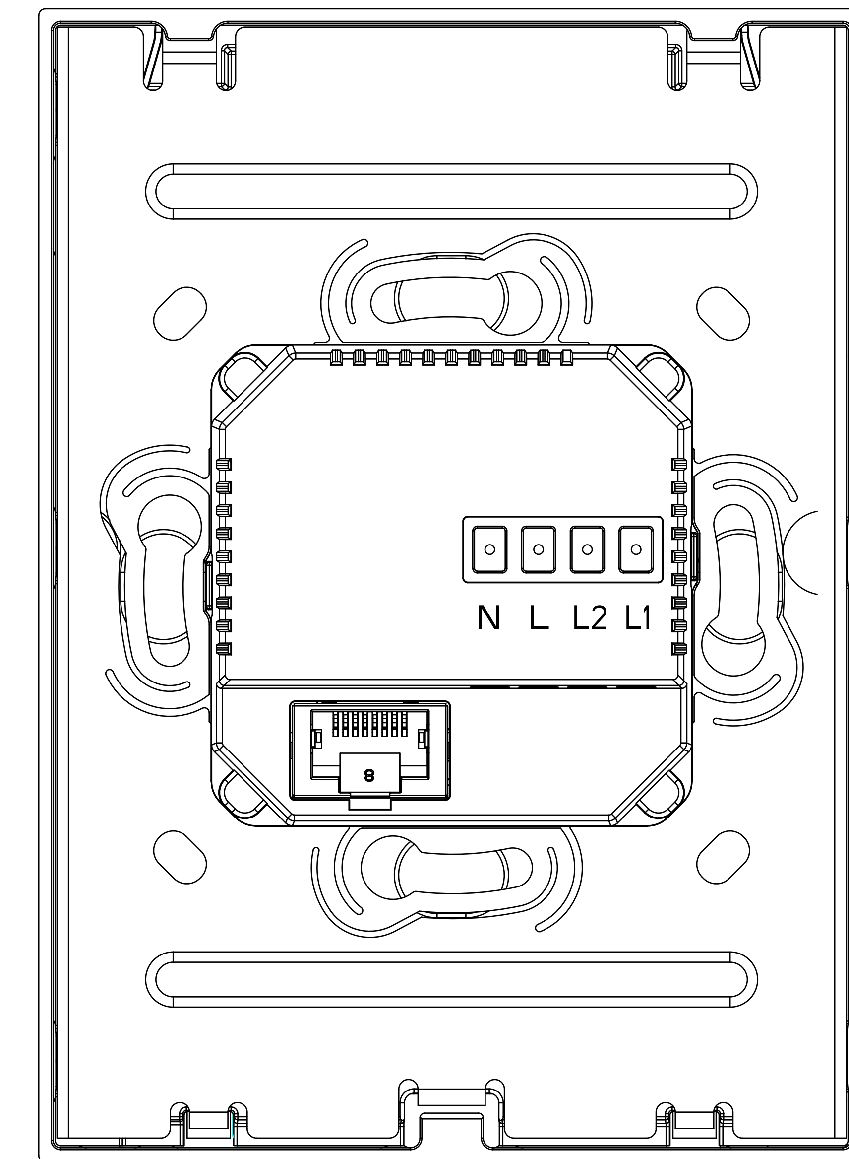
4 BACK VIEW
