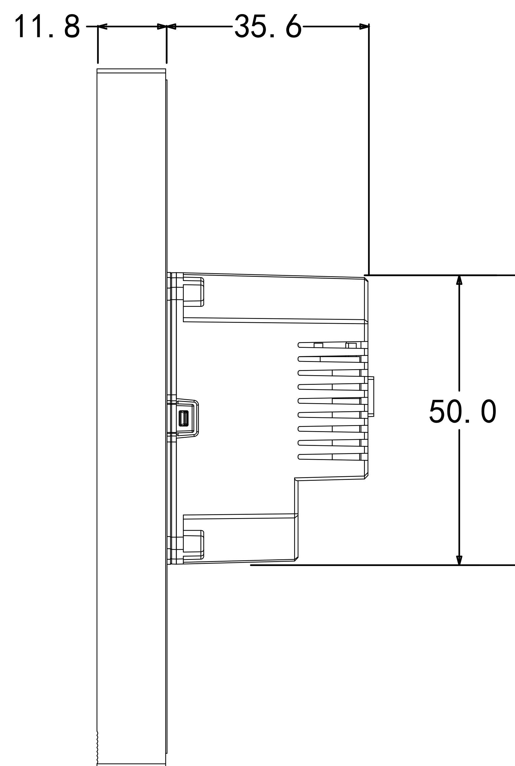
2 RIGHT VIEW
